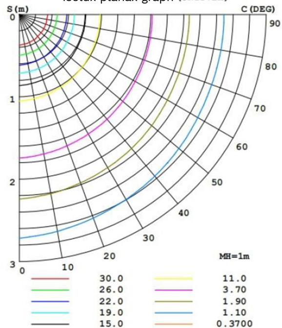
isolux planax graph (UNIT: lx)
