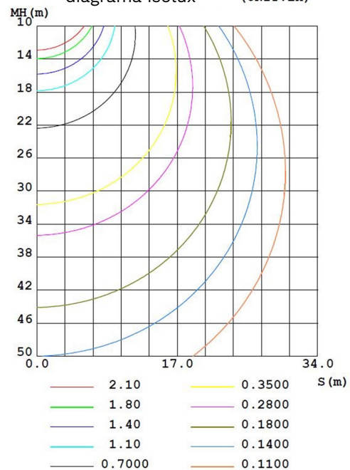
diagrama isolux (UNIT: 1x)
